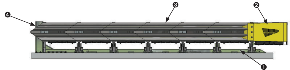
QuadGuard M10 Test Level 3 System
